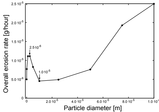
Figure 2. Overall erosion rate vs. particle diameter
